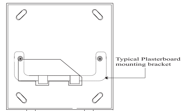
Fix mounting plate to plasterboard
