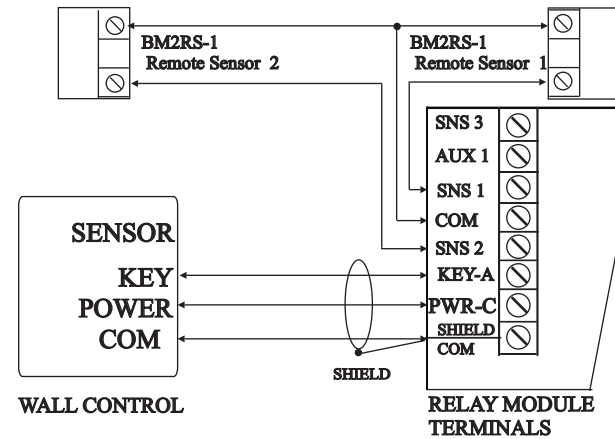
D. Two sensor control. Wall Control sensor not used.
